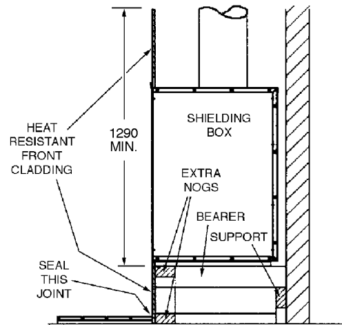
Fig.4 ELEVATED INSTALLATION
